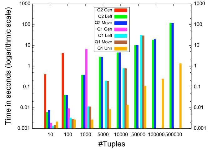
Figure 7: (Synthetic) Varying size of input relation
