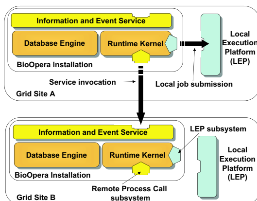
Figure 4. Remote service invocation
