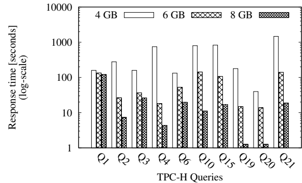
Figure 3. Response time vs. configured DBMS memory
