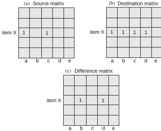
Fig. 3. Source, destination and difference matrices representing a request
