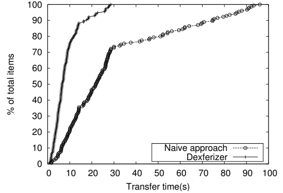
Fig. 7. Comparison of transfer times using Dexferizer and a naive approach.
