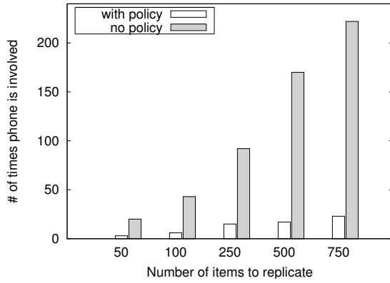
Fig. 8. Transfer policy in action.
