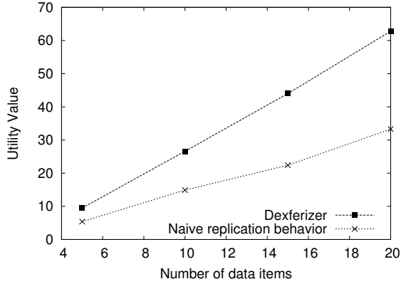
Fig. 6. Utility comparison between optimized versus naive behavior.
