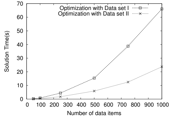
Fig. 10. Performance figure for the vanilla approach.
