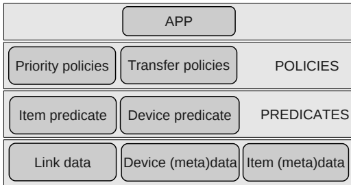
Fig. 5. Declarative transfer service abstraction layers.
