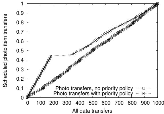
Fig. 9. Priority policy in action.
