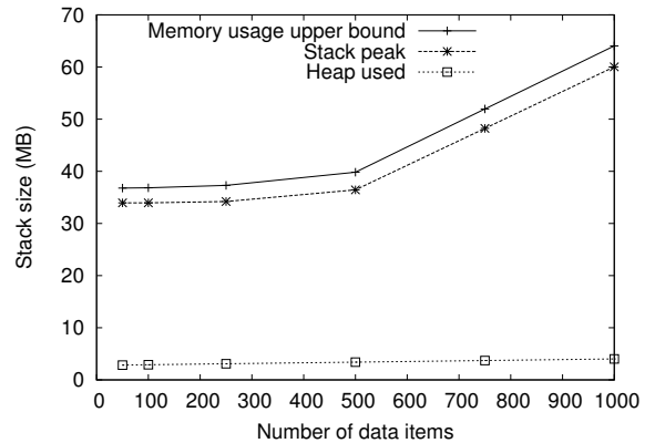
Fig. 11. CLP solver memory consumption.
