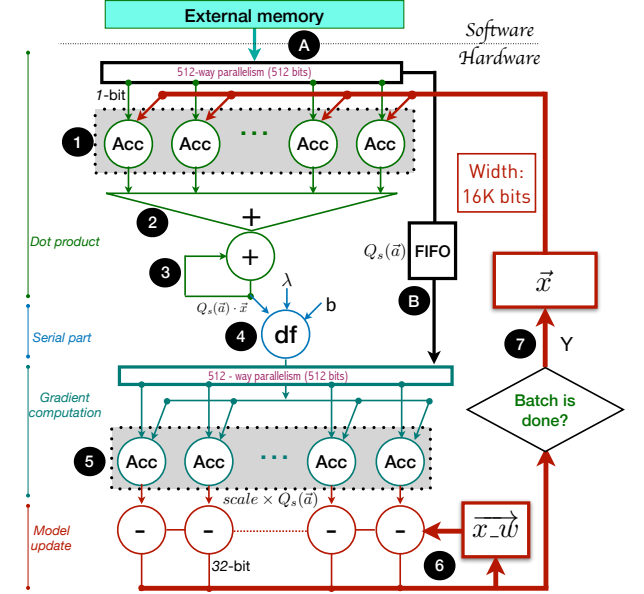
Figure 5: Fully pipelined BWeaving hardware design with 1 bank ( \#Bank = 1 ), according to Algorithm 1.
